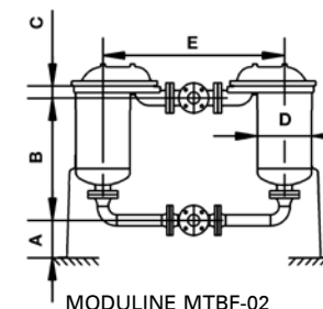
MODULINE MTBF-02
