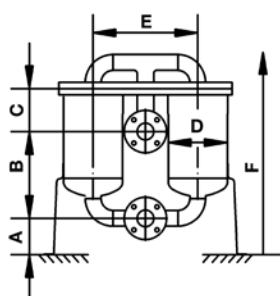
TOPLINE TBF-02
